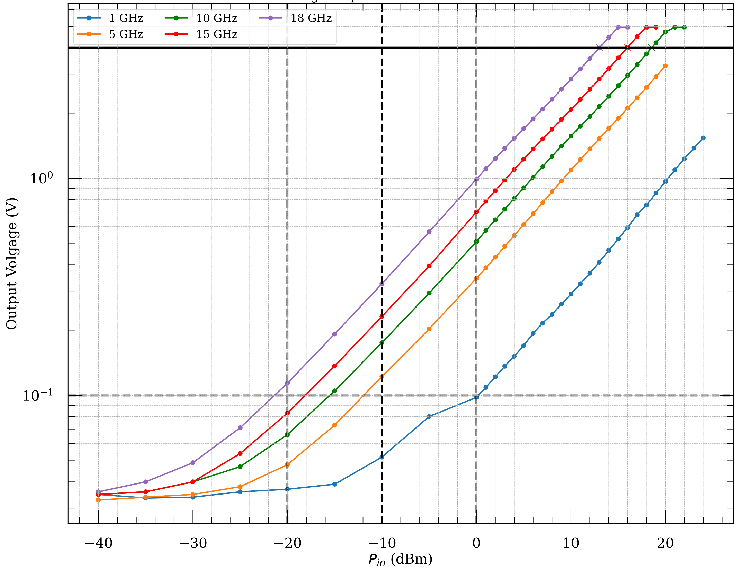
Measured voltage-to-power curve of detector module046
